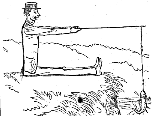
THE RIGHT ANGLE.
