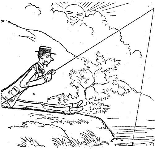
THE ACUTE ANGLE.
