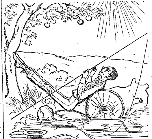
THE ANGLE OF REFLECTION.
